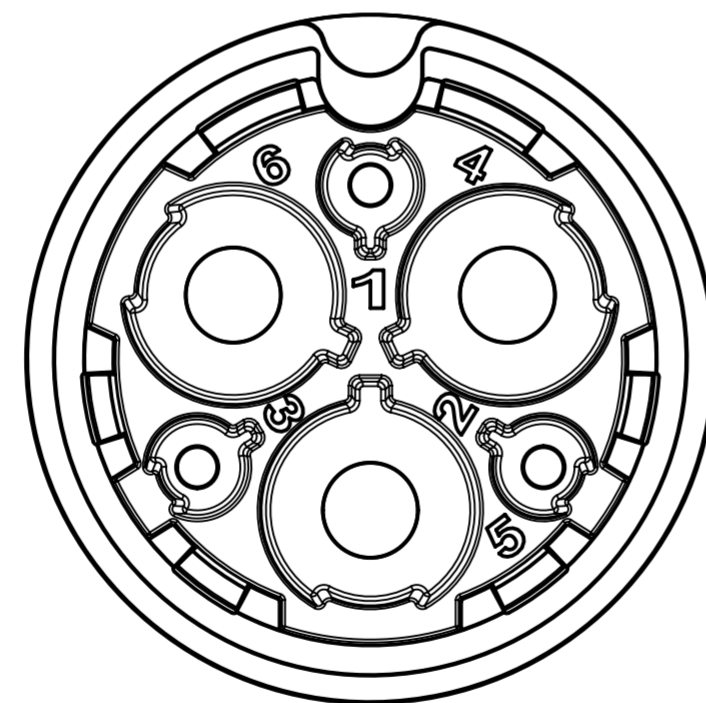
Insulation Body
