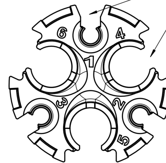
Contact Carrier
