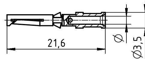
female contact
