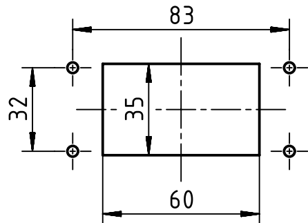
panel cut out (1:2)
